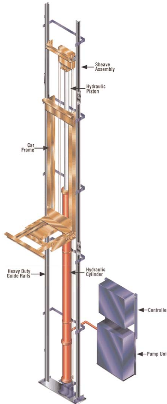
Roped Hydraulic System with Sling
